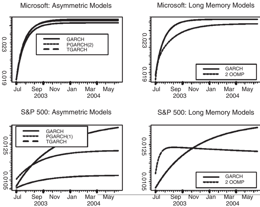
Fig. 9 Predicted Volatility from Competing GARCH Models.
