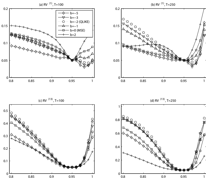
Fig. 3 Plots of size-adjusted power for DMW tests using two different proxies for latent volatility, daily returns squared ( RV^{(1)} ) and 30-minute realised volatility ( RV^{(13)} ). All loss functions are members of the “robust” loss function family, equation (43). Note: The scale of the y-axis changes in each panel.
